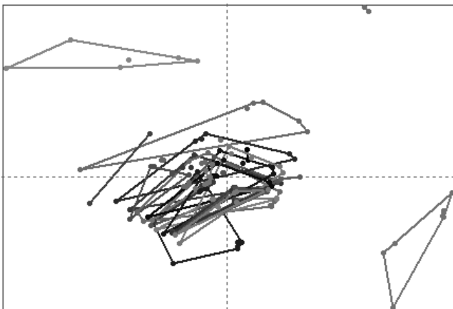
Figure 3. HMDS display for the GCC data set before feature selection. Convex hulls indicate failures involving same defect.
